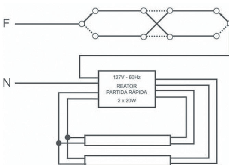
Fig. – Diagrama D4 – Diagrama multifilar
