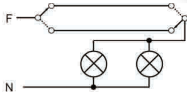
Fig. – Diagrama multifilar do interruptor paralelo ( three-way )
