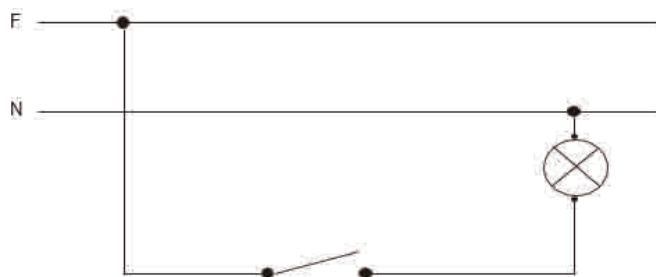
Fig. Diagrama unifilar multifilar
