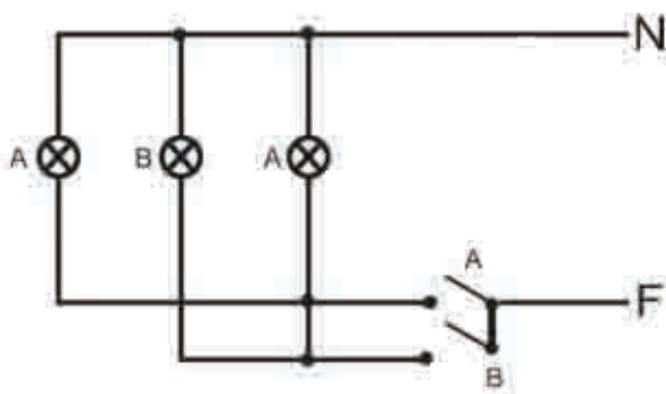
Fig. – Diagrama multifilar
