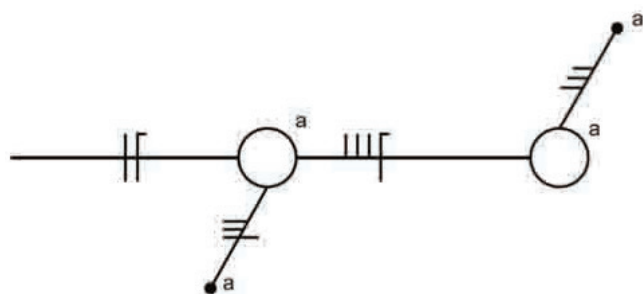
Fig. – Diagrama unilar do interruptor paralelo ( three-way )
