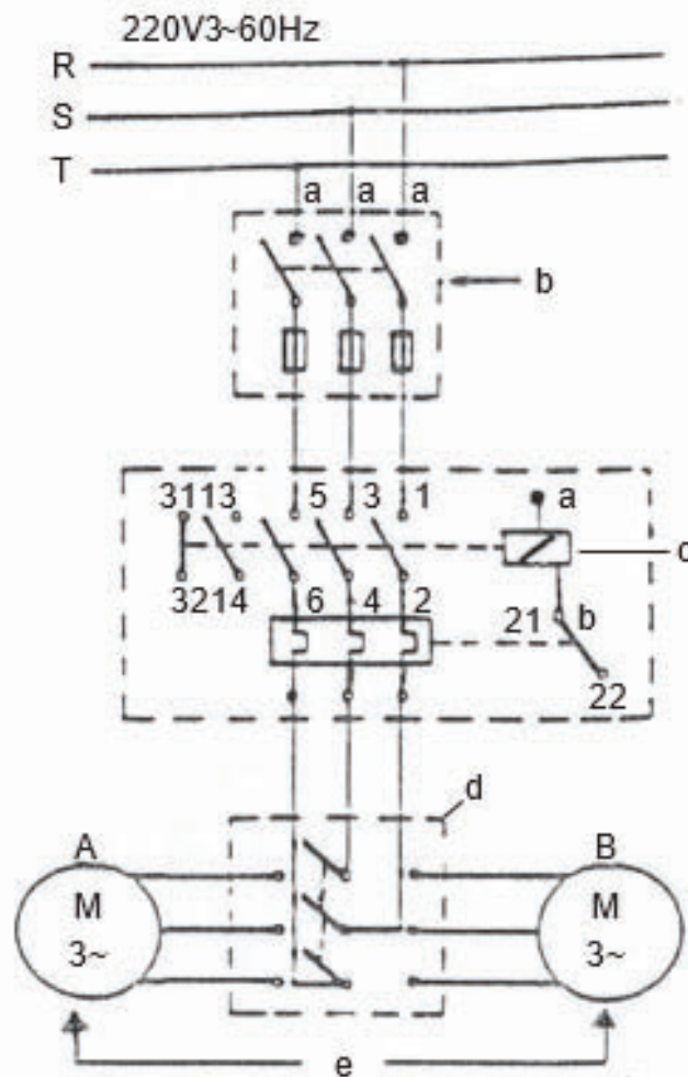
Fig. – Diagrama do circuito principal
